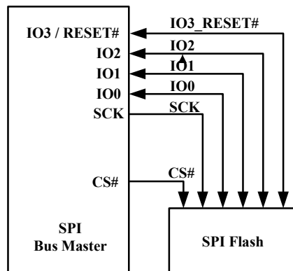
Figure 4. Bus Master and Memory Devices on the SPI Bus - Quad Bit Data Path - I/O3_RESET#
