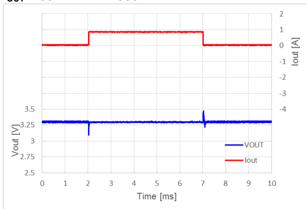
RP602Z330x, V_{IN} = 3.6\text{ V} , MODE = H
