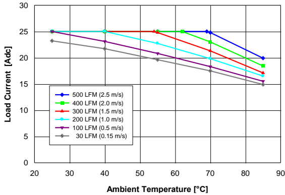
Figure 9. Available load current vs. ambient air temperature and airflow rates for QM48T25050 converter with B height pins mounted vertically with air flowing from pin 3 to pin 1, MOSFET temperature \leq 120^{\circ}\text{C} , V_{in} = 48\text{ V} .
