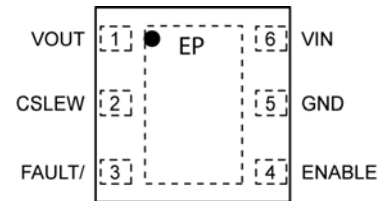
6-Pin MLF ® (ML) (Top View) MIC20X5
