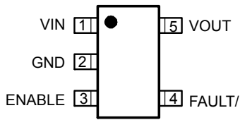
5-Pin SOT-23 (M5) MIC2005-X.XL
