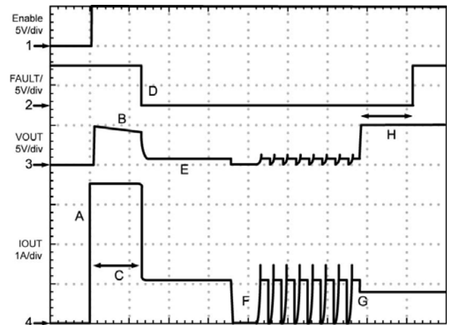
Figure 3. Kickstart™ Operation
