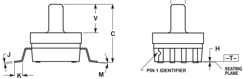
CASE 482A-01 ISSUE A
