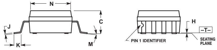
CASE 482-01 ISSUE O
