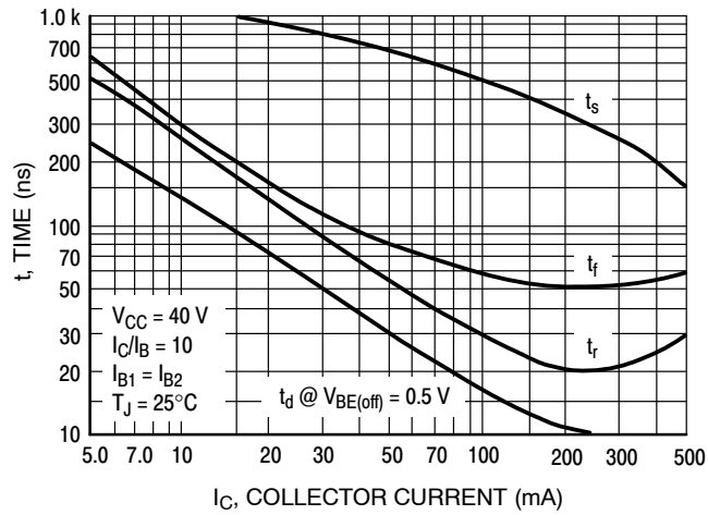
Figure 4. Switching Time
