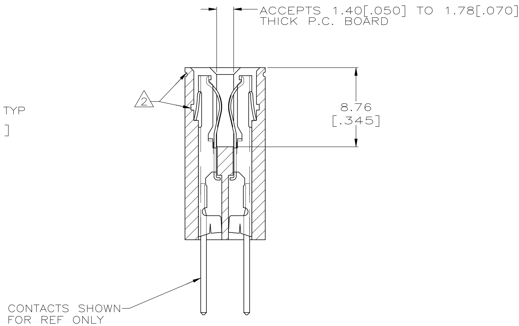
SECTION Z-Z
