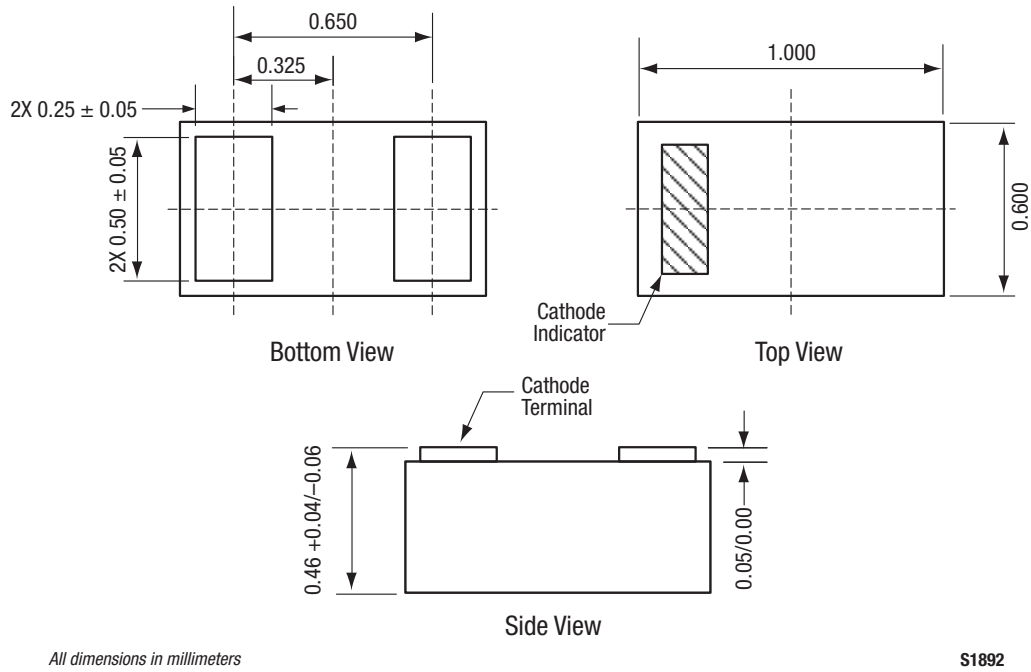
Figure 11. SOD-882 Package Dimension Drawing
