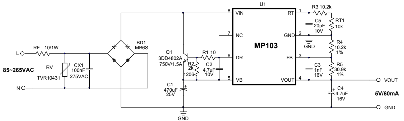
Figure 7: Typical Application
