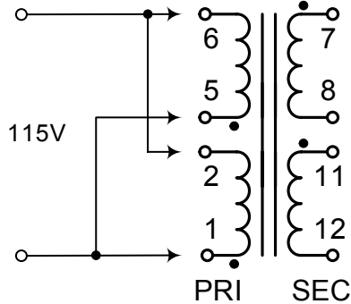
Primary Wiring for 115V (Parallel Connection)
