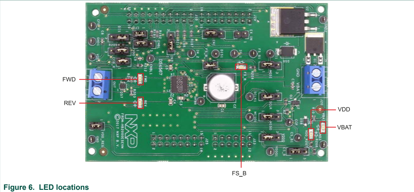
Figure 6. LED locations
