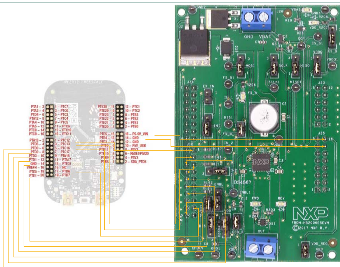
Figure 12. FRDM-KL25Z to FRDM-HB2000ESEVM connections
