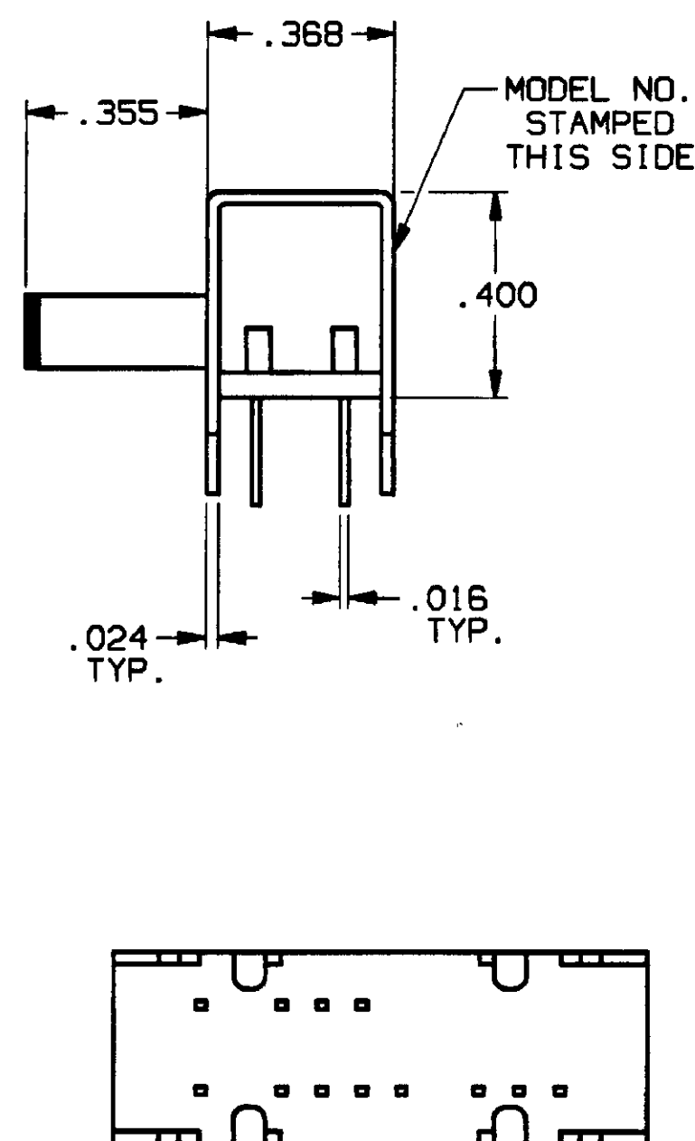
SWITCH BOTTOM VIEW
