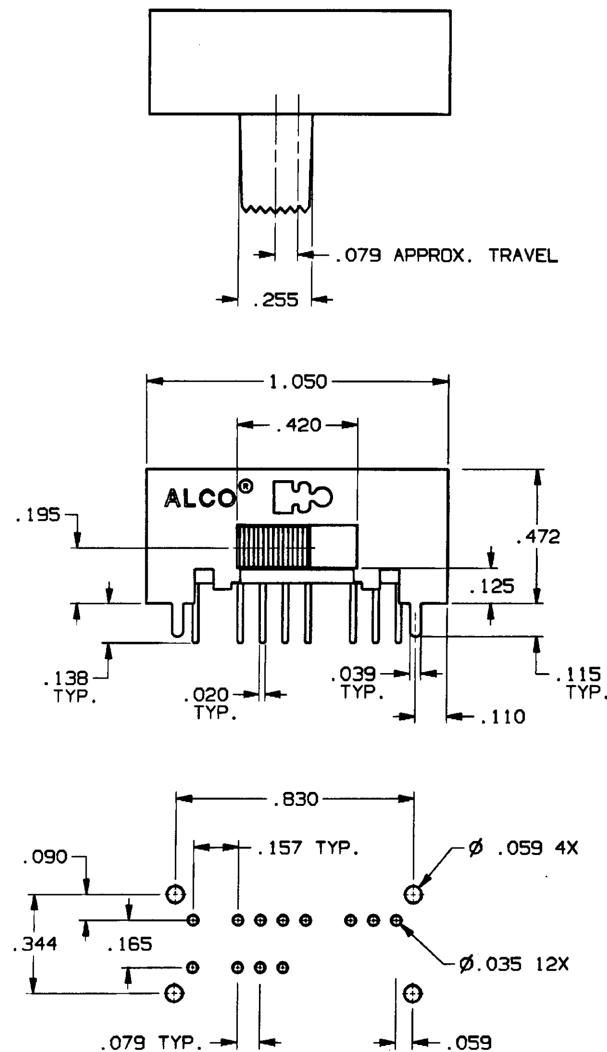
PC HOLE LAYOUT (TOP VIEW) RECOMMENDED TOLERANCES \pm .002
