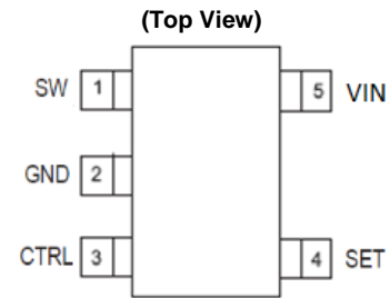
TSOT25 (Top View)
