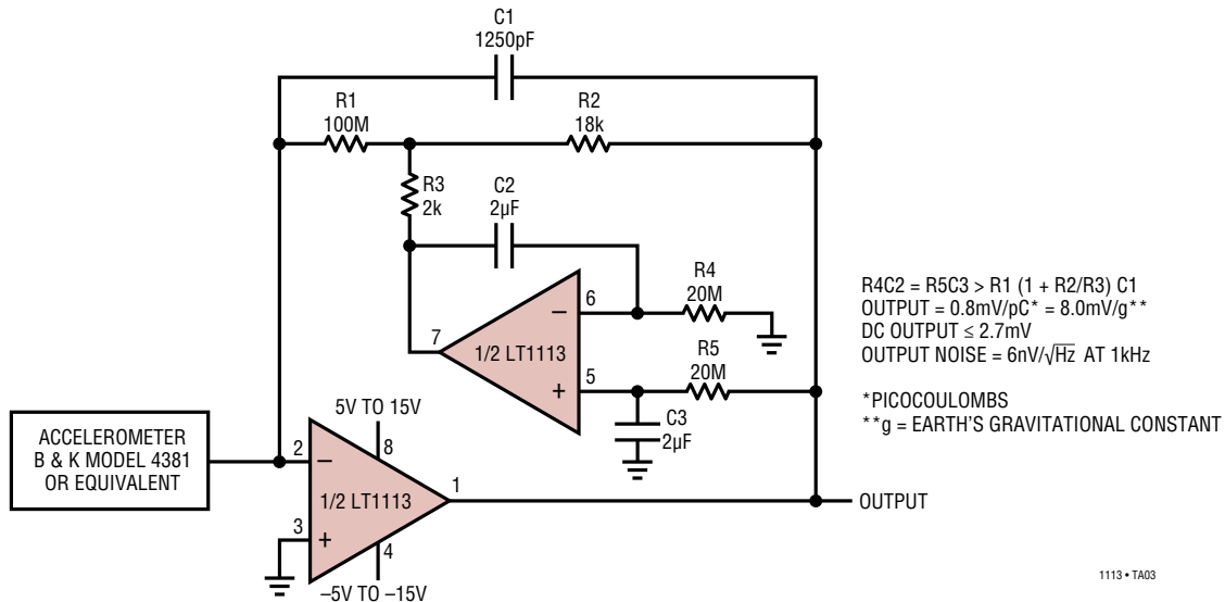
Accelerometer Amplifier with DC Servo
