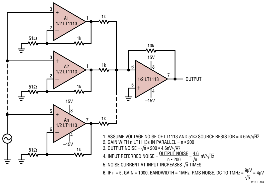
Paralleling Amplifiers to Reduce Voltage Noise
