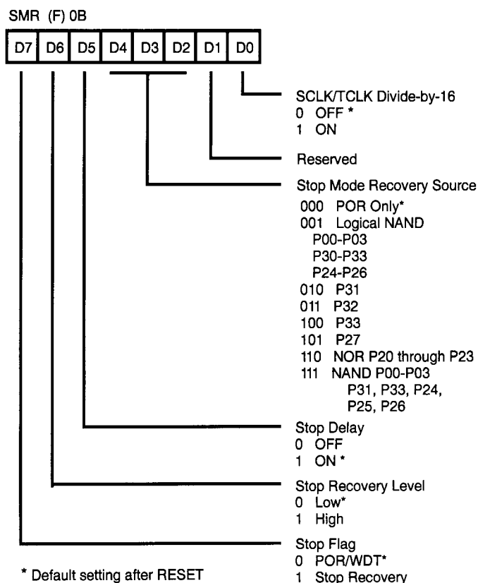
Figure 20. Stop-Mode Recovery Register
