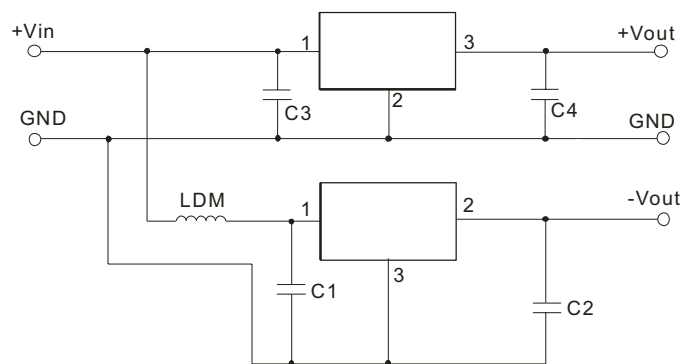
Positive and Negative Output Paralleling Application Circuit
