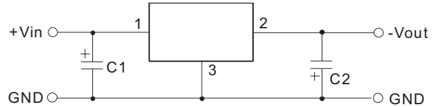
Negative Output Application Circuit
