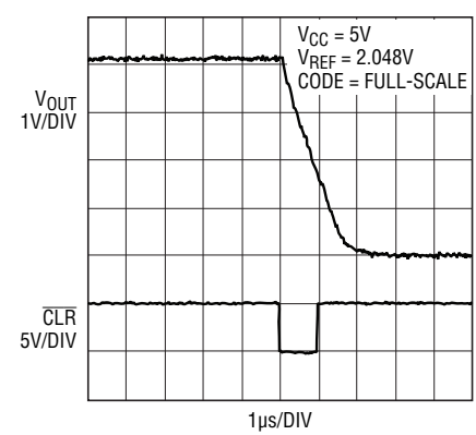
Hardware \overline{\text{CLR}} to Zero-Scale
