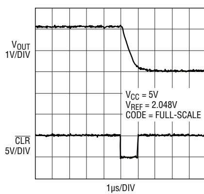
Hardware \overline{\text{CLR}} to Mid-Scale
