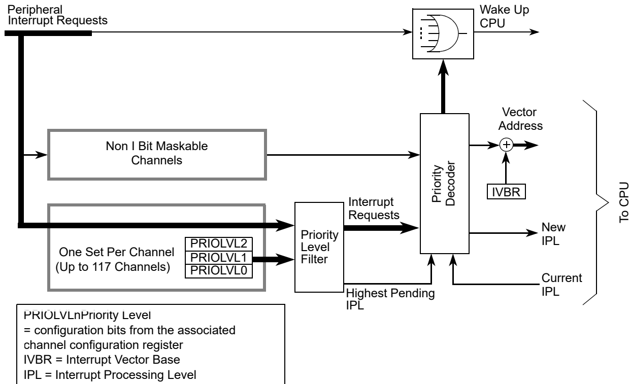
Figure 6-1. S12ZINTV0 Block Diagram
