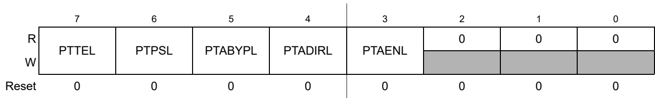
Figure 2-28. Port L Analog Access Register (PTAL)
