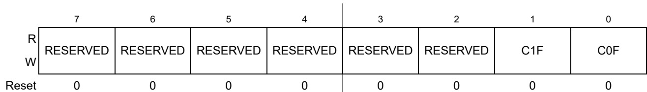
Figure 16-16. Main Timer Interrupt Flag 1 (TFLG1)
