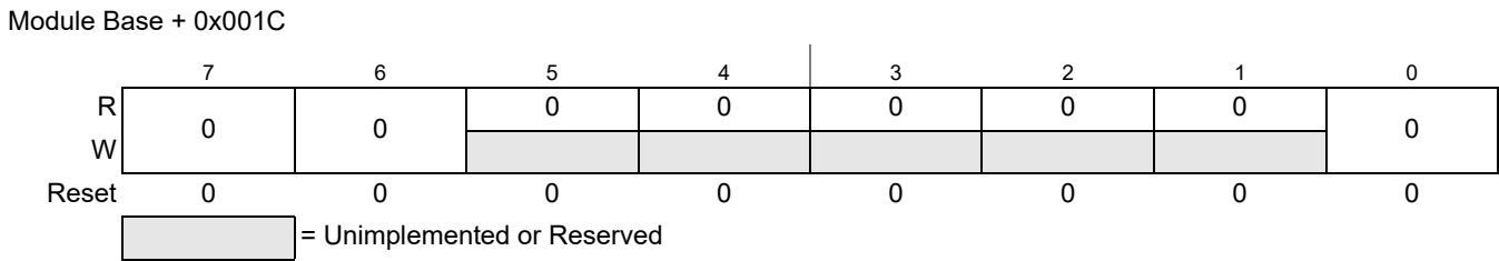
Figure 9-35. Reserved Register CPMUTEST2
