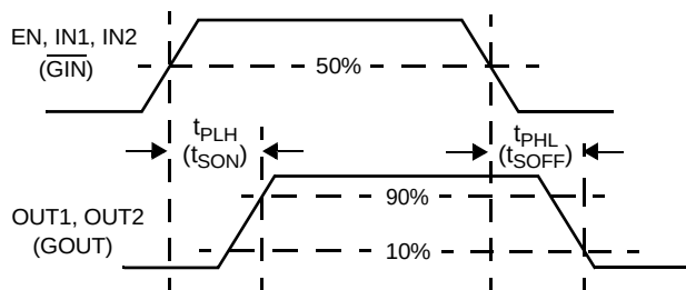
Figure 5. t_{\text{PLH}} , t_{\text{PHL}} , and t_{\text{PZH}} Timing
