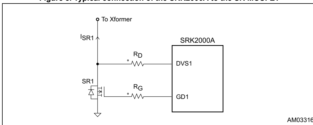
Figure 8. Typical connection of the SRK2000A to the SR MOSFET
