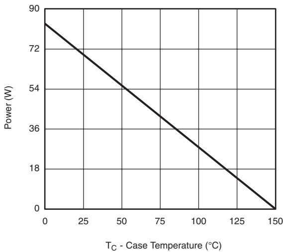
Power, Junction-to-Case
