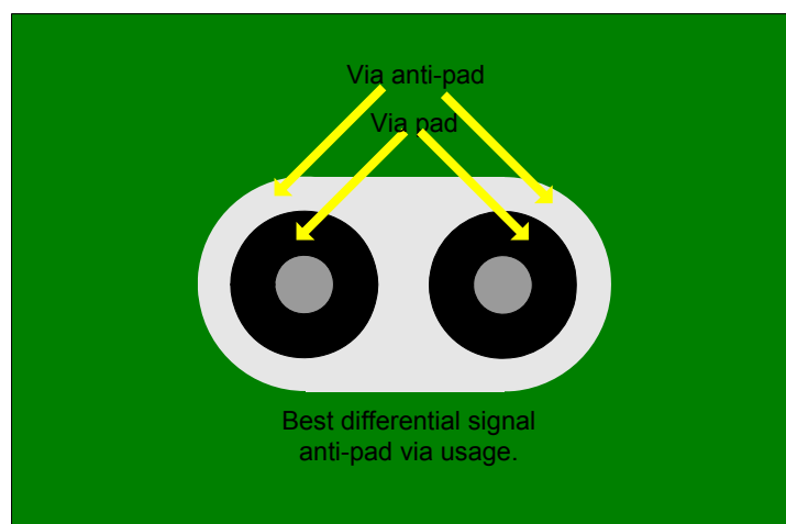
Figure 9-19 Best Differential Signals Via Anti-Pads
