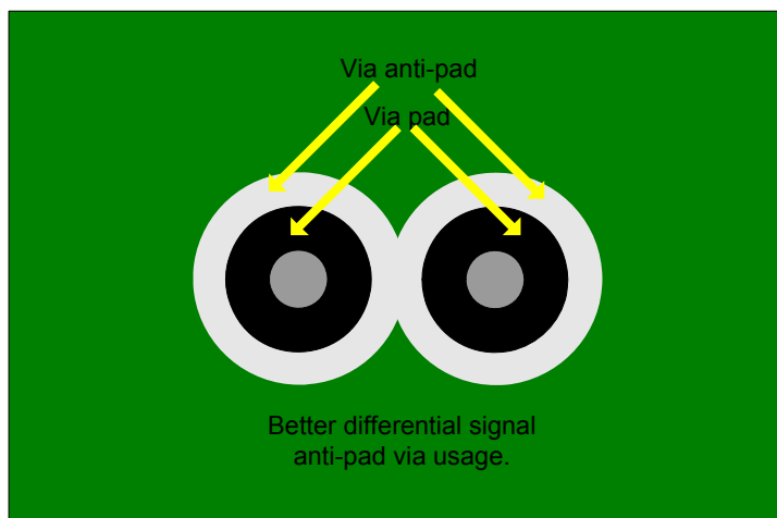
Figure 9-18 Better Differential Signals Via Anti-pads
