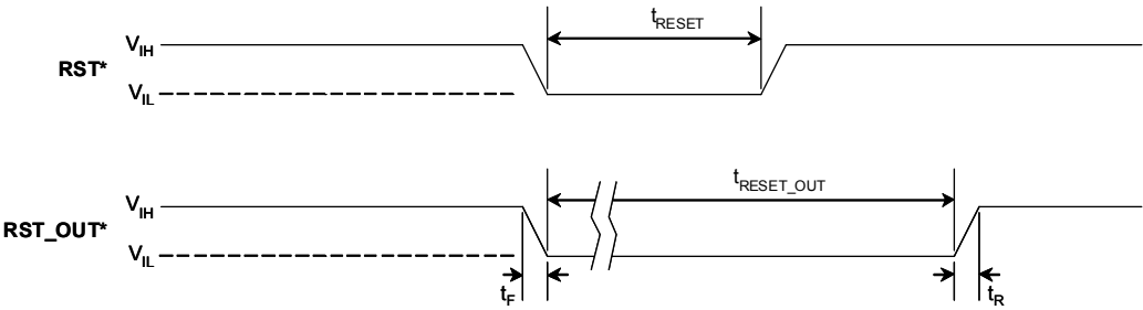
Figure 5-3 Reset Timing Diagram
