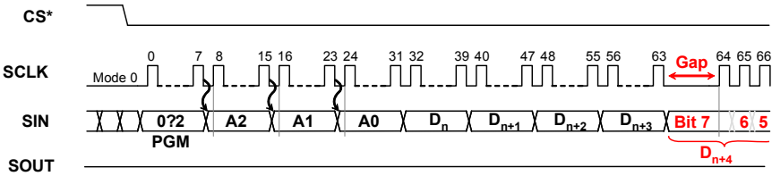
Figure 2-4 SPI Burst Read
