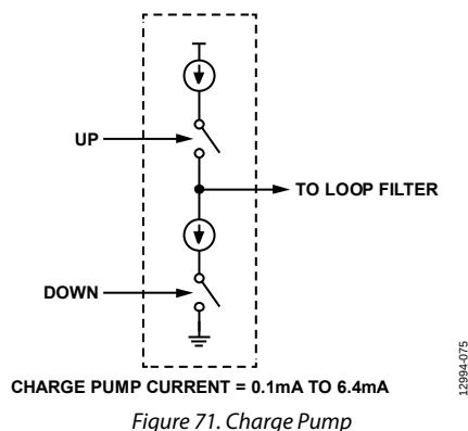
Figure 71. Charge Pump
