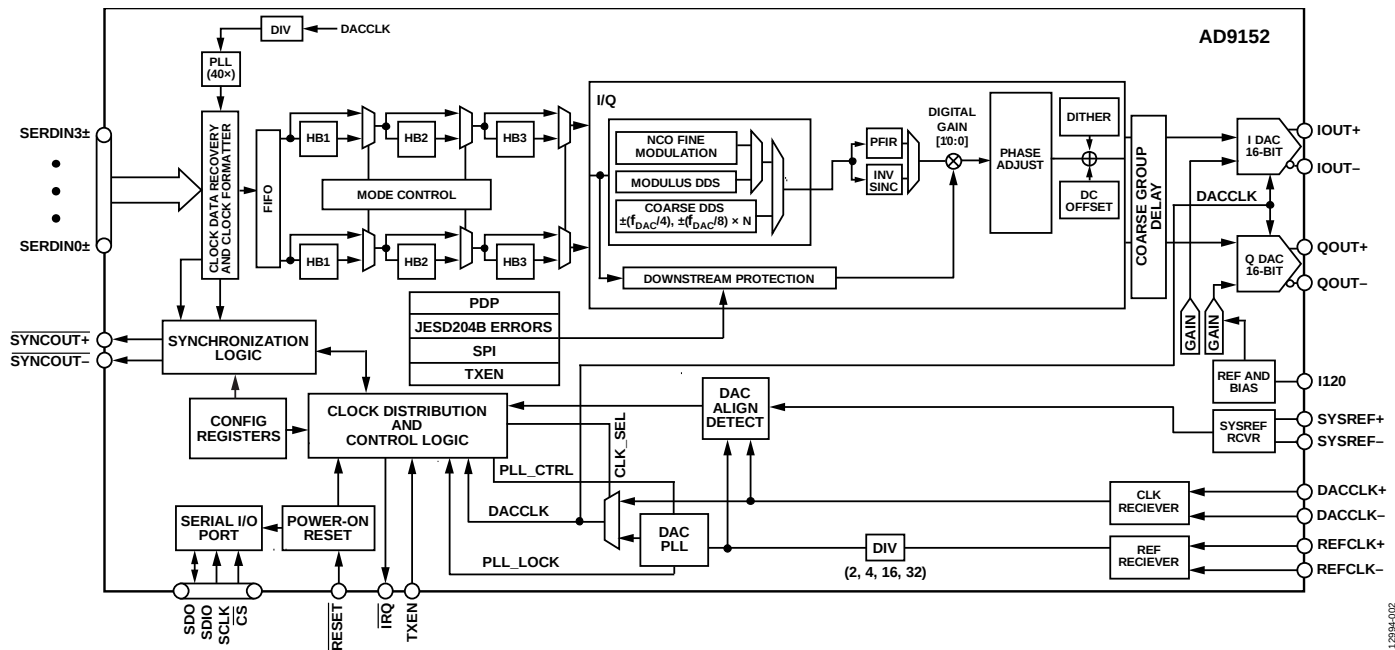
Figure 2. Detailed Functional Block Diagram
