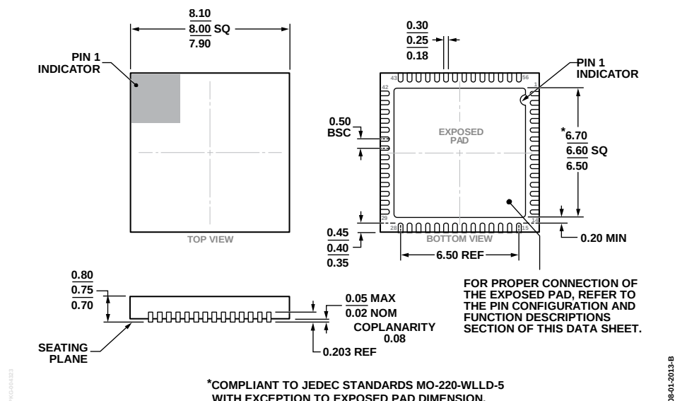
Figure 80. 56-Lead Lead Frame Chip Scale Package [LFCSP_WQ] 8 mm × 8 mm Body, Very Very Thin Quad (CP-56-9)
