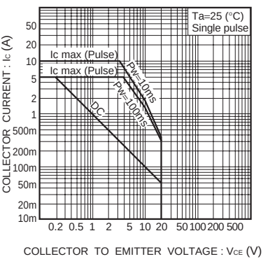
Fig.13 Safe operating area (2SD2118)
