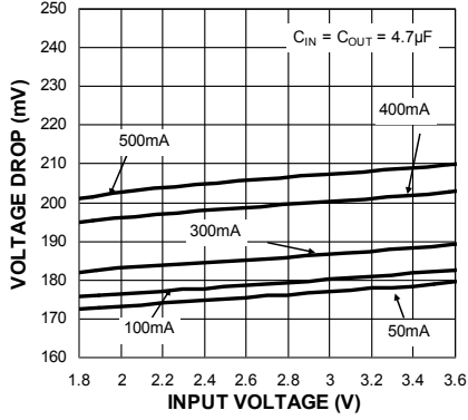
Voltage Drop vs. Input Voltage
