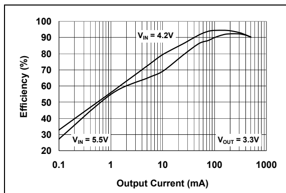
FIGURE 2-10: Efficiency vs. Output Load ( V_{OUT} = 3.3V ).
