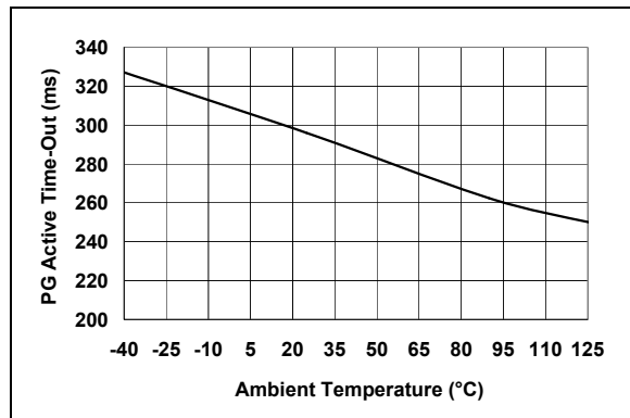
FIGURE 2-8: PG Active Time-out vs. Ambient Temperature.
