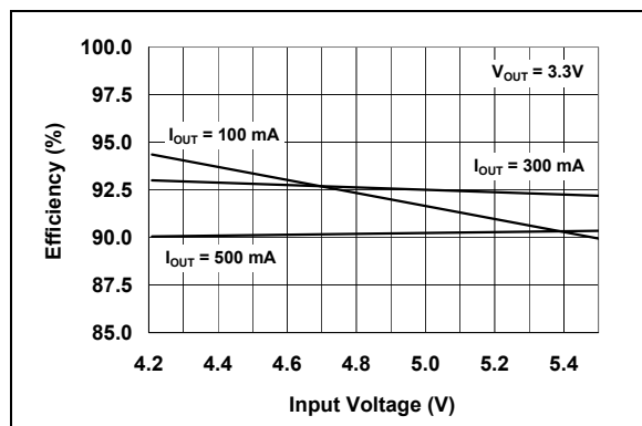
FIGURE 2-7: Efficiency vs. Input Voltage ( V_{OUT} = 3.3V ).
