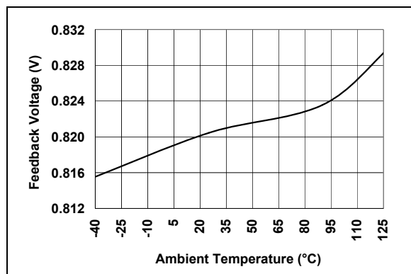
FIGURE 2-9: Feedback Voltage vs. Ambient Temperature.
