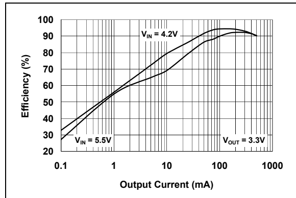
FIGURE 2-10: Efficiency vs. Output Load ( V_{OUT} = 3.3V ).
