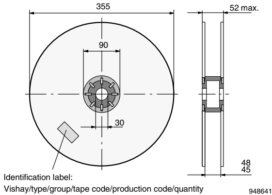
Figure 19. Reel Dimensions
