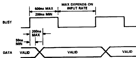
Figure 2. Timing Diagram
