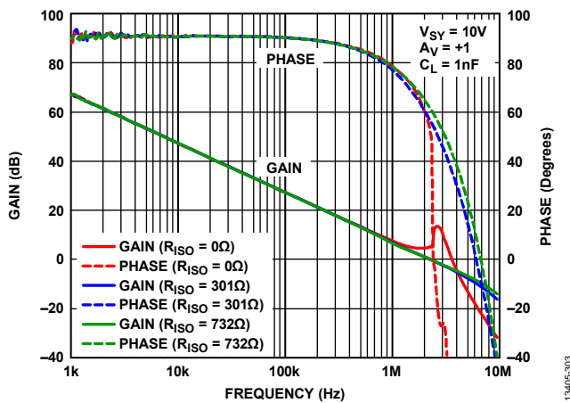
Figure 103. Frequency Response with C_L = 1\text{ nF} and Various Isolating Resistors
