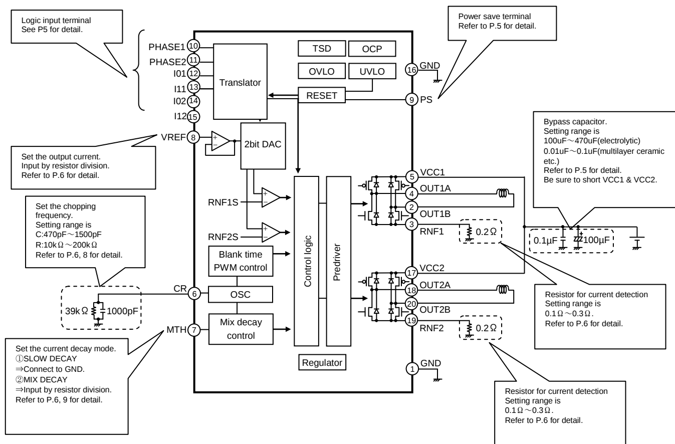
Figure 8. BD68610EFV block diagram and applied circuit diagram
