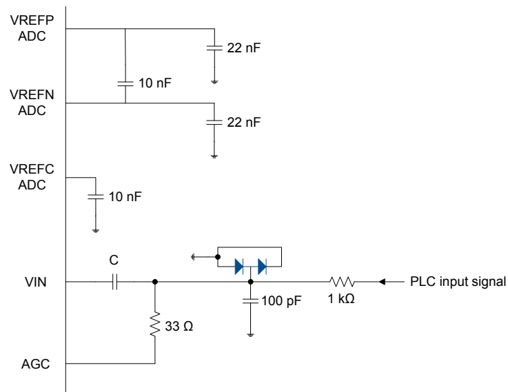
Figure 11-3. Electrical Connections for PLC Reception
