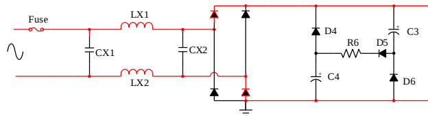
Figure 9: Stage C of Valley Fill Circuit
