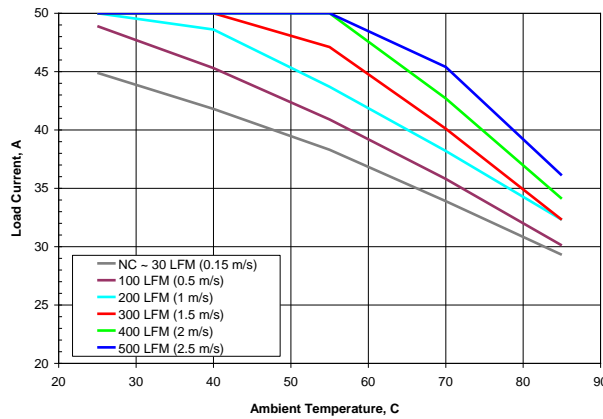
Figure 1. Available load current vs. ambient air temperature and airflow rates for SQE48T50012 converter mounted vertically with air flowing from pin 3 to pin 1, MOSFET temperature \leq 120\text{ }^\circ\text{C} , V_{in} = 48\text{ V} . Note: NC – Natural convection
