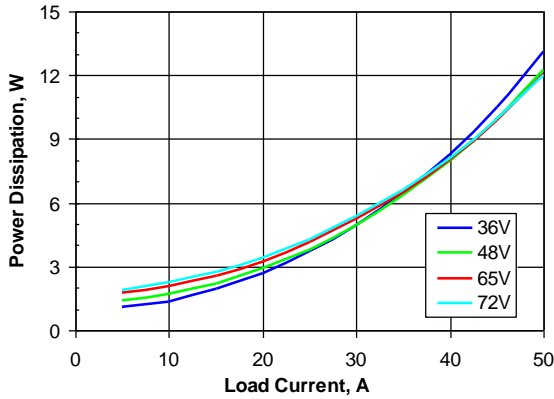
Figure 4. Power dissipation vs. load current and input voltage for SQE48T50012 converter mounted vertically with air flowing from pin 3 to pin 1 at a rate of 300 LFM (1.5 m/s) and T_a = 25\text{ }^\circ\text{C} .
