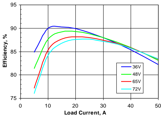
Figure 2. Efficiency vs. load current and input voltage for SQE48T50012 converter mounted vertically with air flowing from pin 3 to pin 1 at 300 LFM (1.5 m/s) and T_a=25\text{ }^\circ\text{C} .
