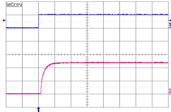
Figure 7. Turn-on transient at full rated load current (resistive) plus 10,000\text{ }\mu\text{F} at V_{in} = 48\text{ V} , triggered via ON/OFF pin. Top trace: ON/OFF signal (5 V/div.). Bottom trace: Output voltage (0.5 V/div.). Time scale: 5 ms/div.
