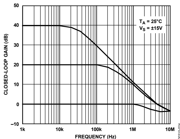
Figure 24. OP292/OP492 Closed-Loop Gain vs. Frequency @ ±15 V
