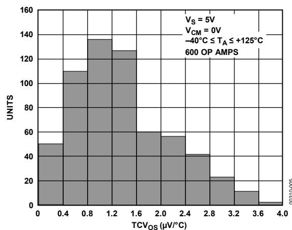
Figure 5. OP292 Temperature Drift ( \text{TCV}_{\text{OS}} ) Distribution @ 5 V
