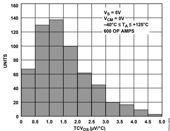
Figure 8. OP492 Temperature Drift ( \text{TCV}_{\text{OS}} ) Distribution @ 5 V
