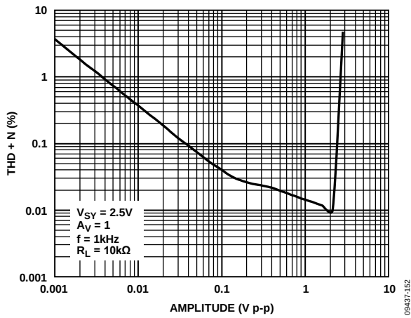
Figure 56. THD + N vs. Amplitude
