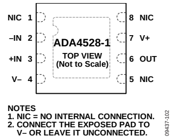
Figure 5. ADA4528-1 Pin Configuration, 8-Lead LFCSP
