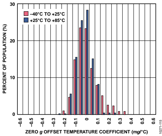
Figure 16. X-Axis Zero g Offset Temperature Coefficient, V_S = 3.0\text{ V}
