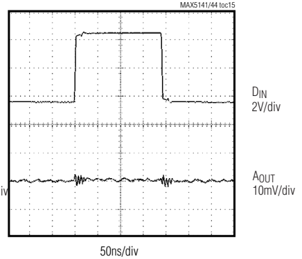
DIGITAL FEEDTHROUGH
