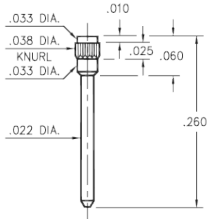
7827-0-00-XX-00-00-03-0 Press-fit in .035 mounting hole
