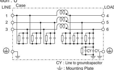
(4) Line to ground capacitor code : 155, 335 Option : U
