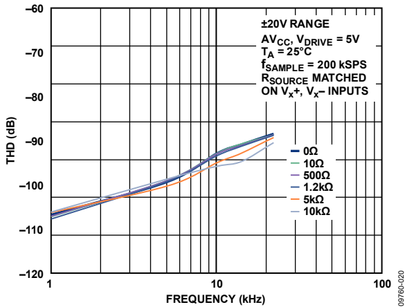
Figure 21. THD vs. Input Frequency for Various Source Impedances, ±20 V Range
