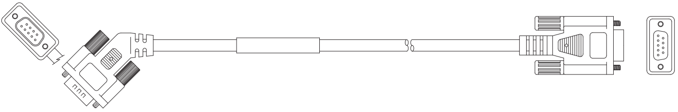
Interface Cable Assembly P28256-MXX
