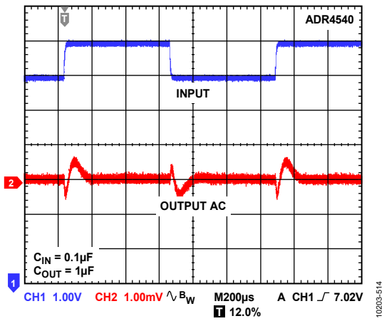
Figure 66. ADR4540 Line Transient Response
