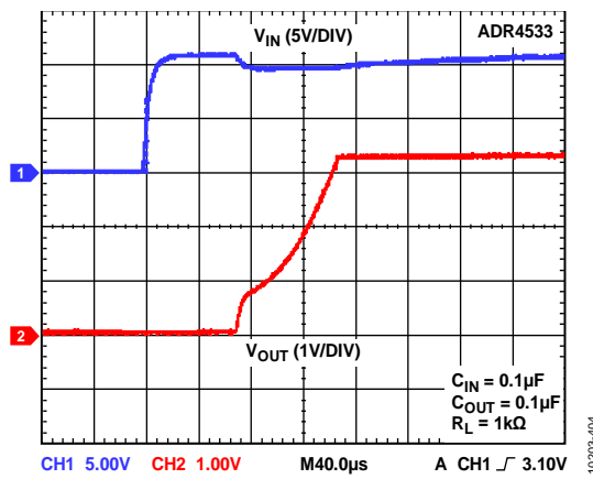
Figure 44. ADR4533 Output Voltage Start-Up Response
